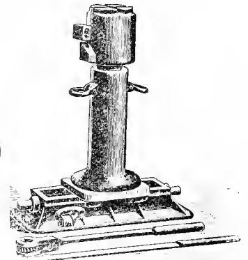
Fig. 3742. TRAVERSING HYDRAULIC JACK.
